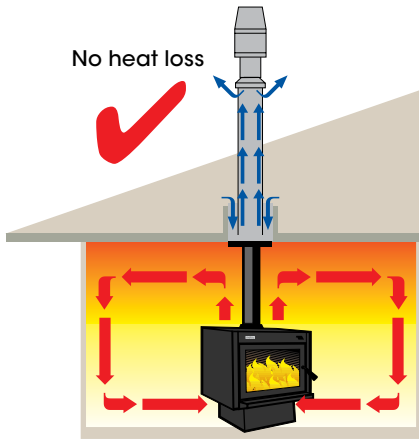
ECO Flue System (ceiling cavity)
