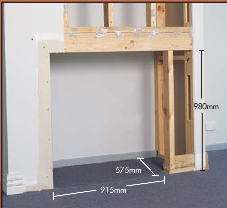
Timber framework, partially plaster board clad
